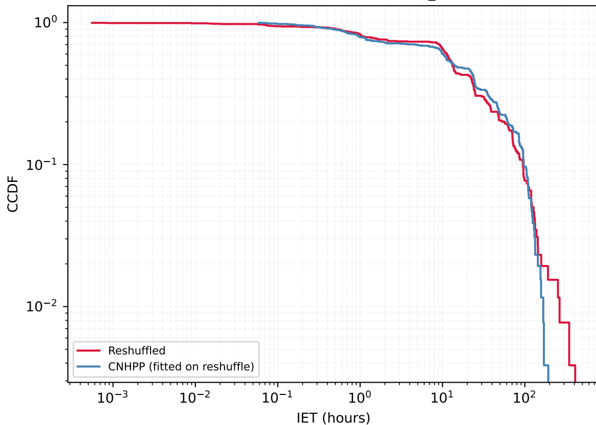
User 8786749 - Reshuffled vs CNHPP A_{\text{fit}}=0.2181
